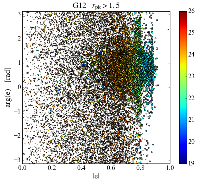
Figure D4. Sources from patch G12 that fail the asteroid cut, plotted in polar ellipticity coordinates ( |e|, \arg(e) ). These sources are at least 1.5 magnitudes brighter in r than in g and in i . Each symbol is colour-coded by the catalogue r magnitude, and the symbol size is proportional to lensfit weight.
