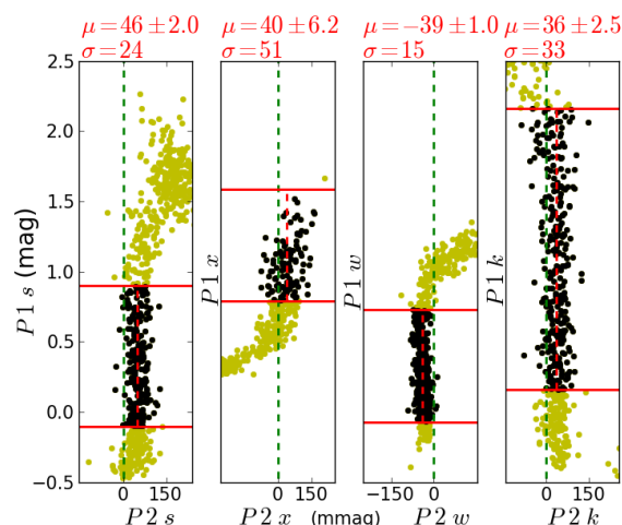
Figure B1. Principal colours s , w , x and k for the pointing KiDS.3.6–34.1. The initial selection of stars (in yellow) is identical for s , w , x and k . From this parent sample the stars on the locus are selected (black). The inferred median P2 offsets, its formal error and the standard deviation of the locus point sources are shown above each panel.
