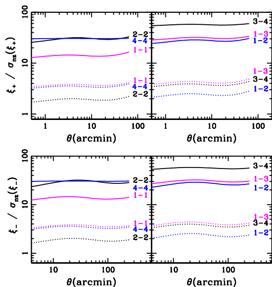
Figure C1. Redshift distribution uncertainty: signal-to-noise estimates of \xi_+ (upper) and \xi_- considering only the statistical noise \sigma_{\text{nz}} that arises from the uncertainty in the n(z) as measured by the weighted direct calibration (DIR, solid) and by the cross-correlation calibration (CC, dotted). This can be compared to the actual signal-to-noise on measurements of \xi_{\pm} in the KiDS-450 data that are presented in Fig. 4 for the same sample of tomographic bins, labelled ‘ i - j ’ where i, j = 1 \dots 4 .
